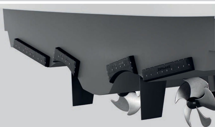
TUNNEL-SHAPED INTERCEPTORS
